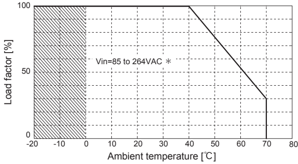
● PCA1000F-5, -12, -15 Ambient Temperature Derating Curve
