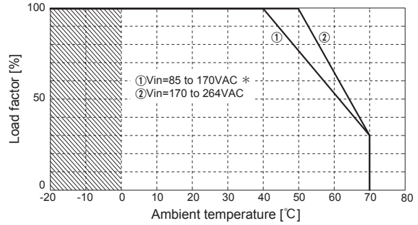
● PCA1000F-24, -32, -48 Ambient Temperature Derating Curve
