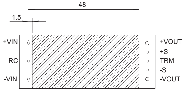
(e) CHS300/CHS380
